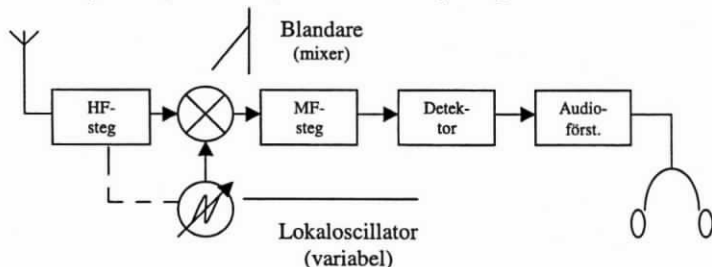
Fig 1, Superheterodynmottagare, blockschema
